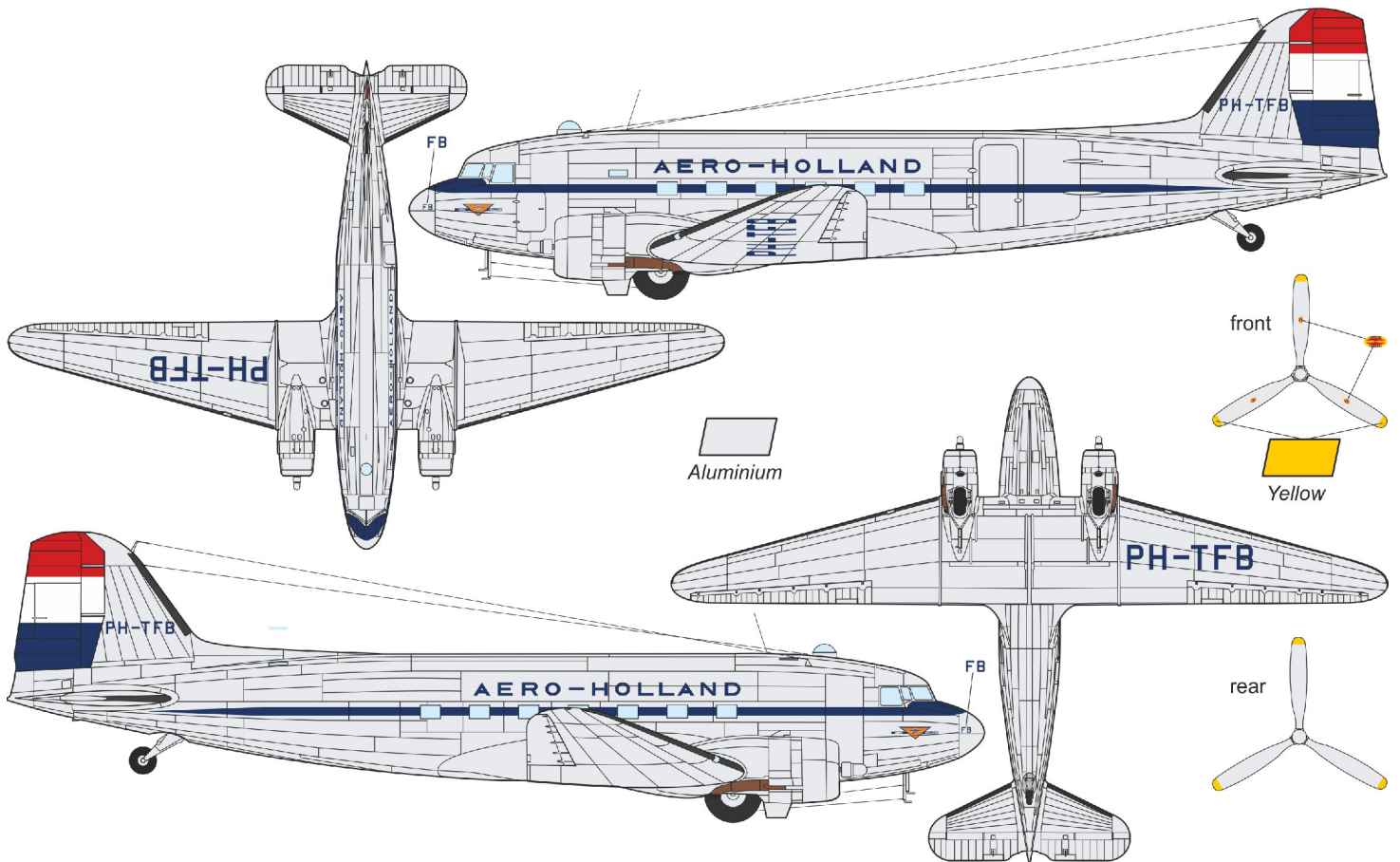
D Douglas C-47A-1-DK, s/n 42-92378, PH-TFB, Aero-Holland N.V., Ypenburg Airport, the Netherlands, 1948-50
