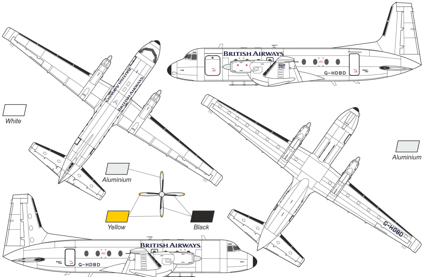
A British Aerospace BAe.748 (Srs.2B Model 378), G-HDBD (c/n 1797), British Airways Ltd., flown between various regional airports, U.K., 1990-92
