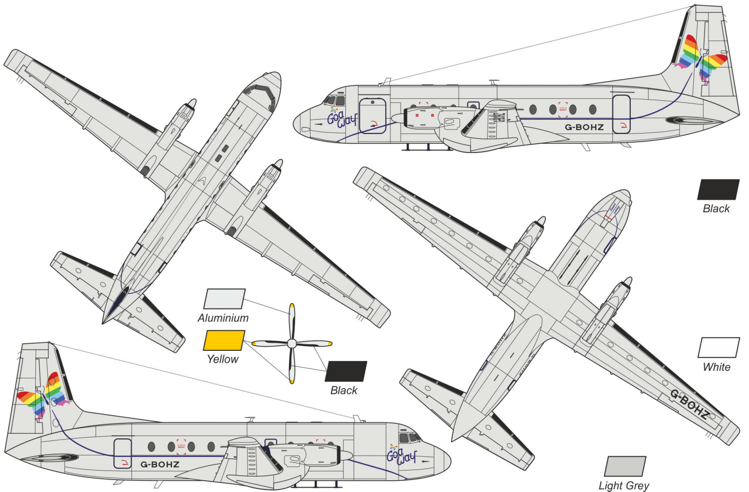
C Hawker Siddeley HS.748 (Srs.2B Model 378), G-BOHZ (c/n 1785), for service with Goa Way Aviation (India's Holiday Airline), Prestwick Airport, Scotland, U.K., 1993-94
