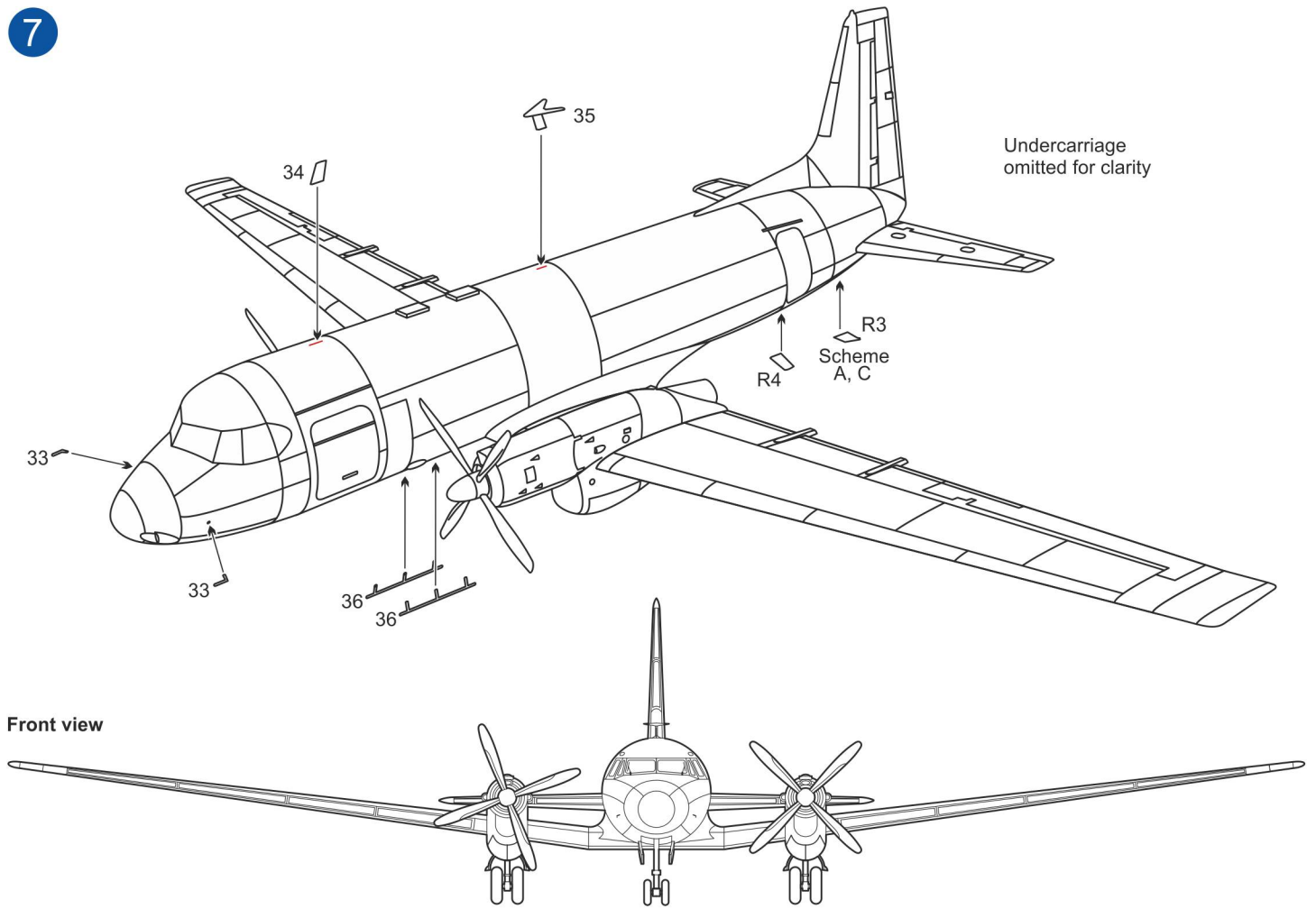
A British Aerospace BAe.748 (Srs.2B Model 378), G-HDBD (c/n 1797), British Airways Ltd., flown between various regional airports, U.K., 1990-92
