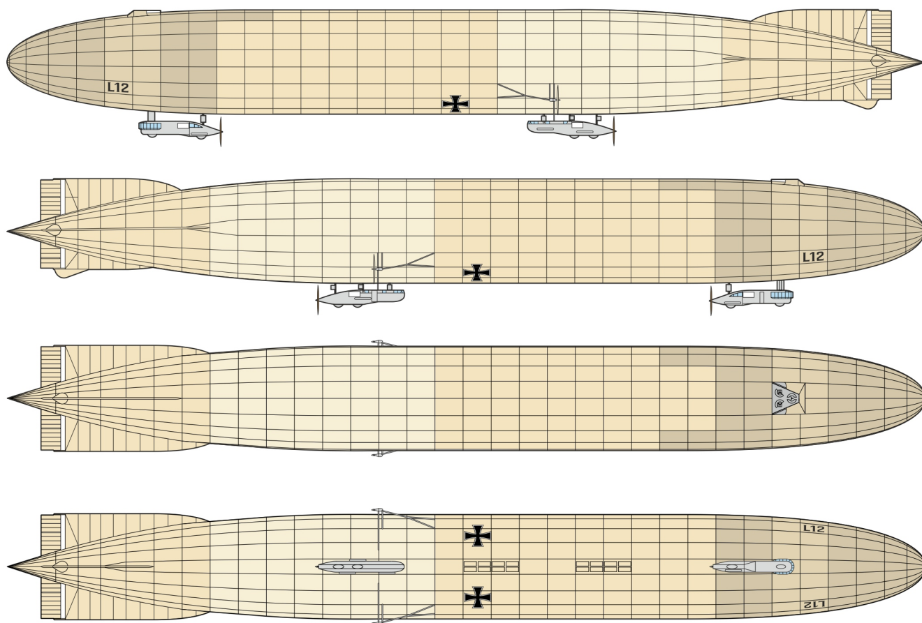
A Zeppelin LZ43 (P-class), L12, Black L12, Naval Airship Division (Marine-Luftschiff-Abteilung), Imperial German Navy (Kaiserliche Marine), Hage Airship Base, Germany, July 1915
