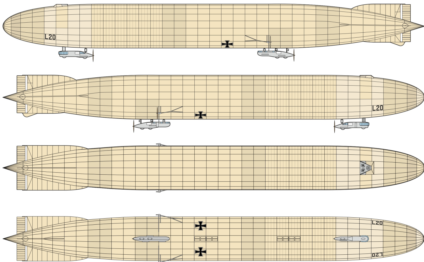
C Zeppelin LZ59 (Q-class), L20, Black L20, Naval Airship Division (Marine-Luftschiff-Abteilung), Imperial German Navy (Kaiserliche Marine), Tondern Airship Base, Germany, April 1916
