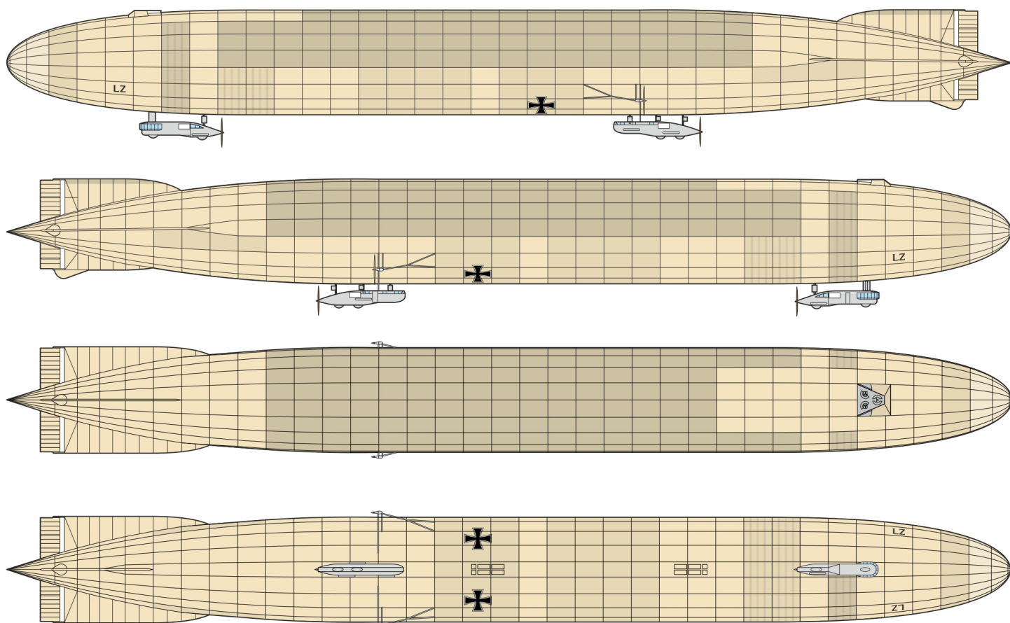
D Zeppelin LZ73 (Q-class), LZ103, Black LZ, Airship Troop (Luftschifftruppe), Imperial German Flying Corps (Fliegertruppe des deutschen Kaiserreiches), Königsberg Airship Base, East-Prussia, Germany (now Kaliningrad, Russia), August 1917
