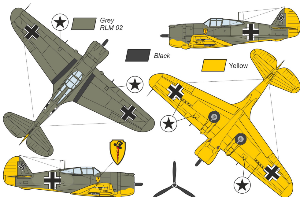
D Curtiss H-75A-1, Jagdfliegerschule 1 (JFS 1) Fighter Training School, Luftwaffe, Werneuchen airfield, Germany, spring 1941
