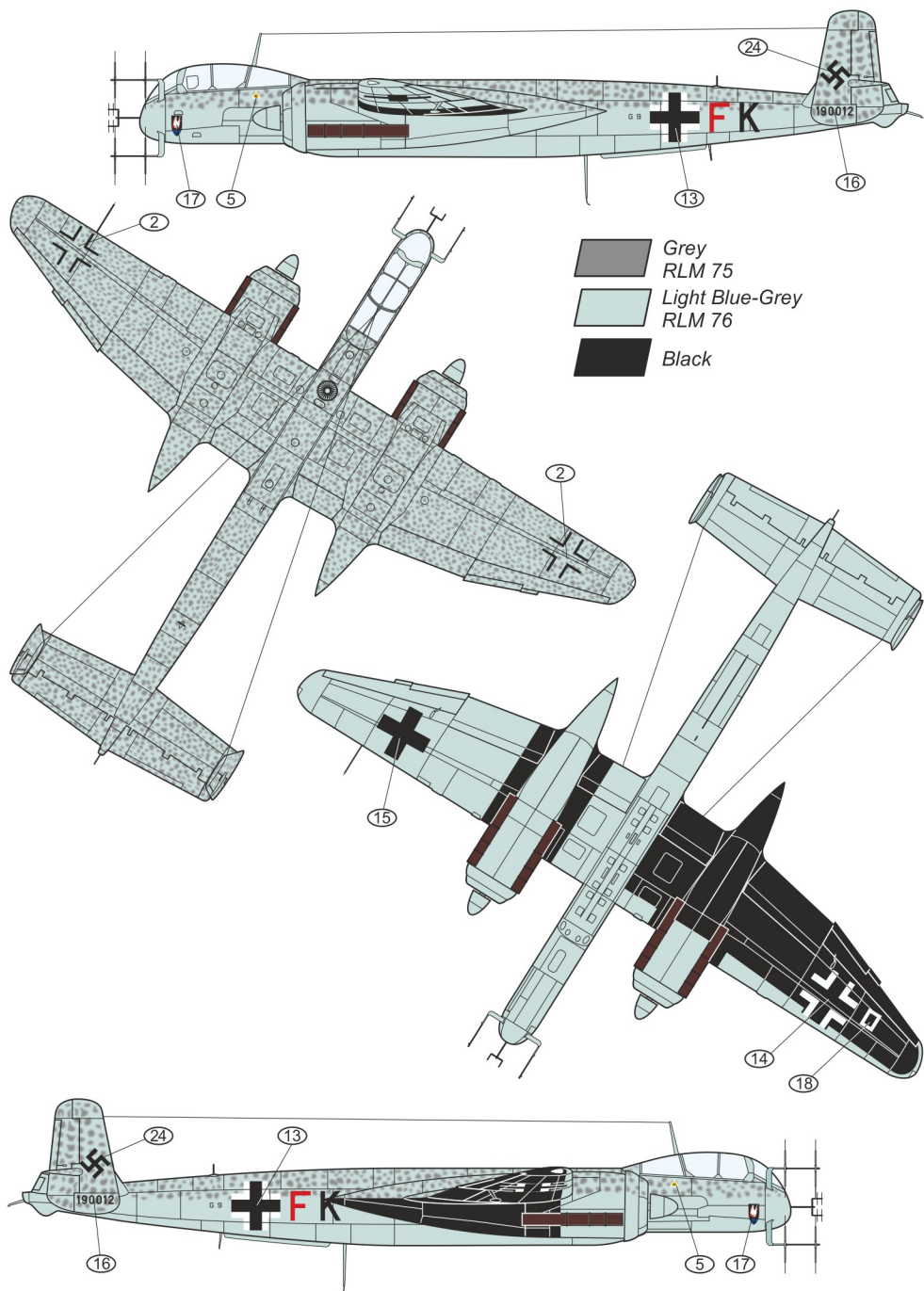
Heinkel He 219A-0/R6, G9+FK (W.Nr. 190012), 2./NJG 1, Luftwaffe, Venlo-Herongen airfield, the Netherlands, April 1944
