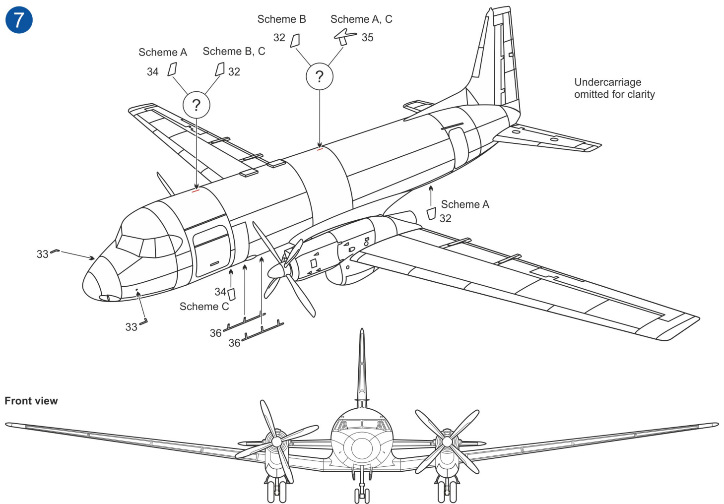
A Hawker Siddeley HS.748 (Srs.2 Model 206) Andover CC Mk.2, XS789 (c/n 1561), No.32 Sq., Royal Air Force, Northolt Air Base, Greater London, U.K., early 1990s
