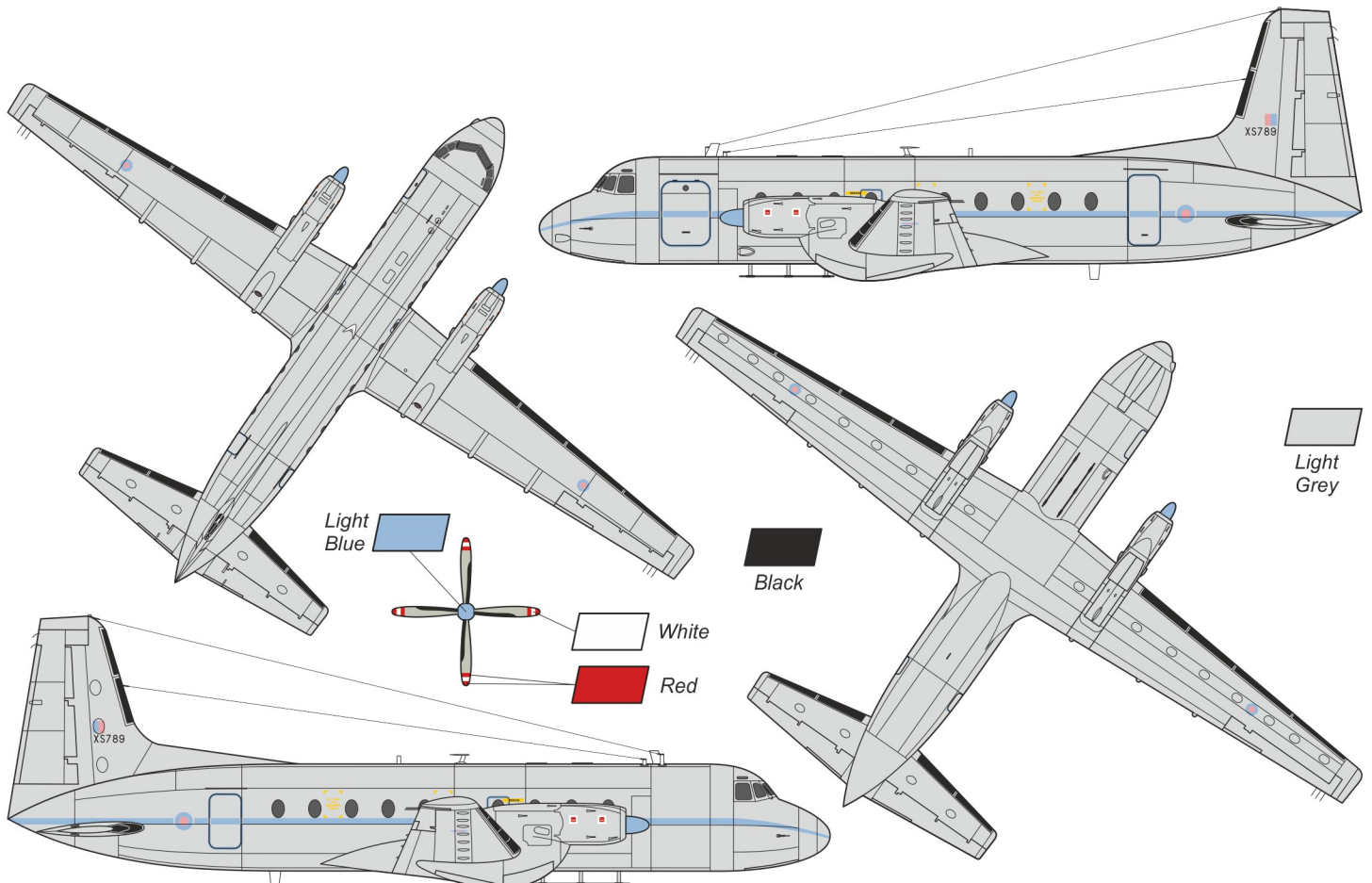
A Hawker Siddeley HS.748 (Srs.2 Model 206) Andover CC Mk.2, XS789 (c/n 1561), No.32 Sq., Royal Air Force, Northolt Air Base, Greater London, U.K., early 1990s
