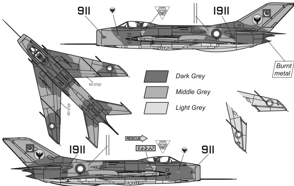
B Shenyang F-6 Farmer C, Black 1911, No.19 'Phoenix' Air Superiority Sq., Pakistani Air Force, Masroor Air Base, 1984
