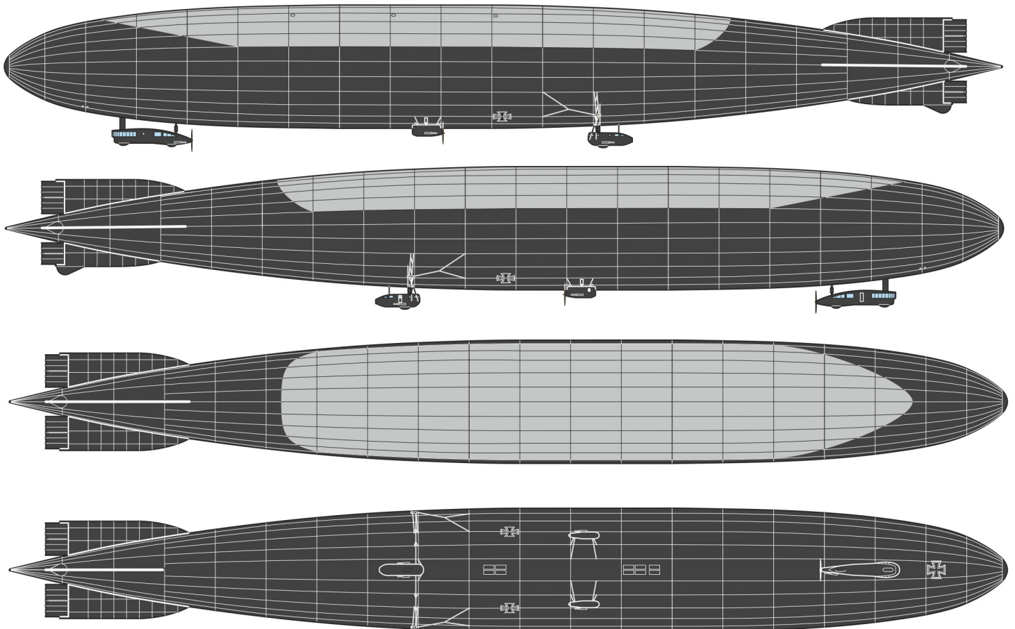
D Zeppelin LZ85 (R-class), L45, Naval Airship Division (Marine-Luftschiff-Abteilung), Imperial German Navy (Kaiserliche Marine), Tønder Airship Base, Denmark, spring 1917
