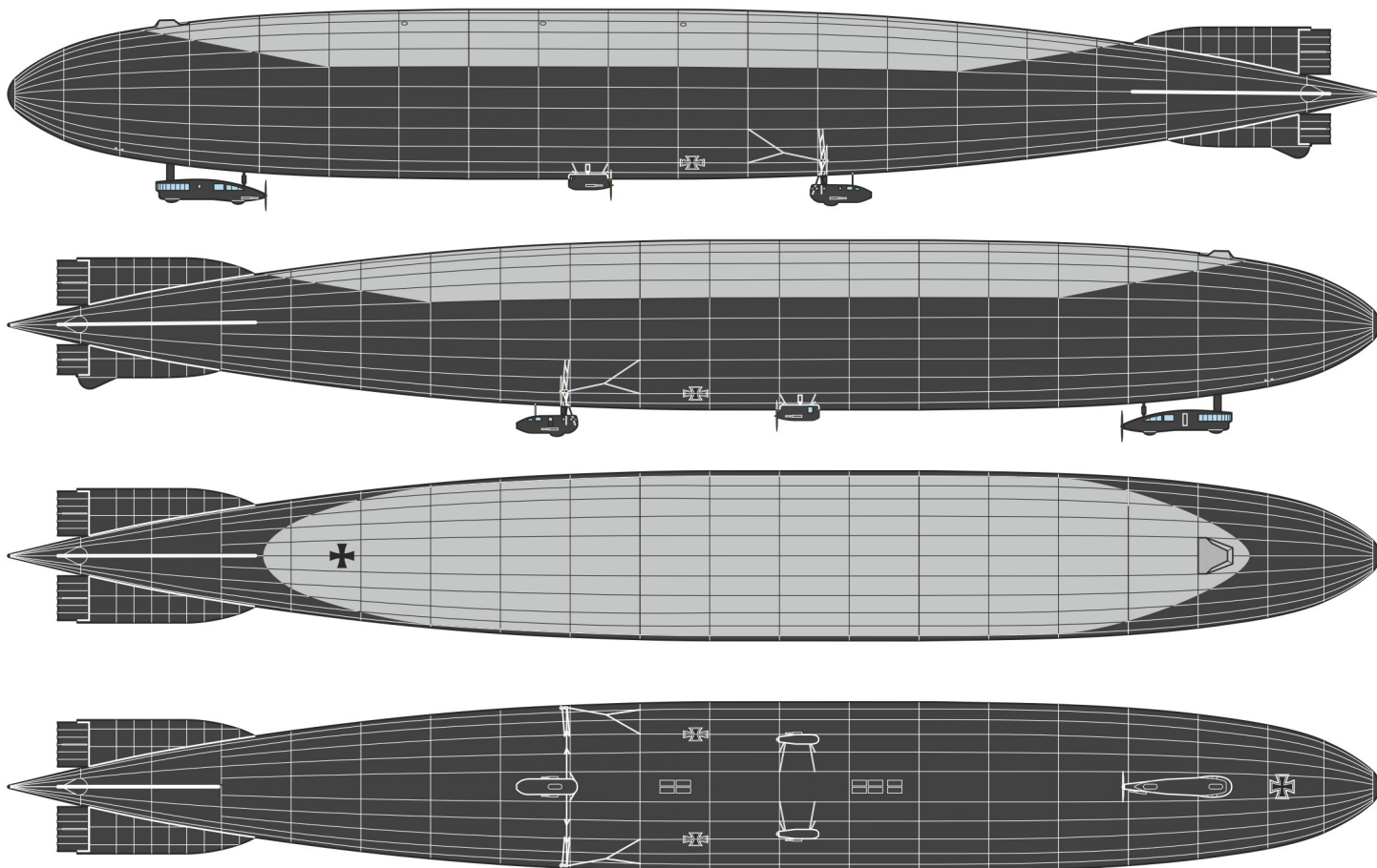
B Zeppelin LZ87 (R-class), Naval Airship Division (Marine-Luftschiff-Abteilung), Imperial German Navy (Kaiserliche Marine), Ahlhorn Airship Base, Germany, November 1917
