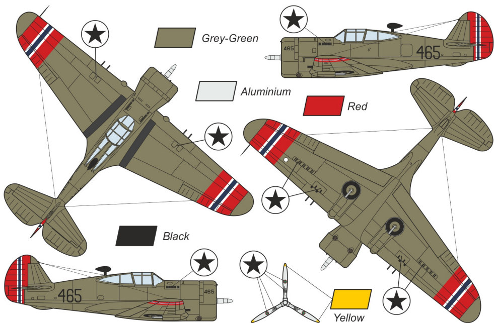
B Curtiss H-75A-8, No. 465, 'Little Norway' Air Force Training Camp, Norwegian Army Air Service (Hærens flyvåpen), Toronto Island Airport, Ontario, Canada, 1942-43
