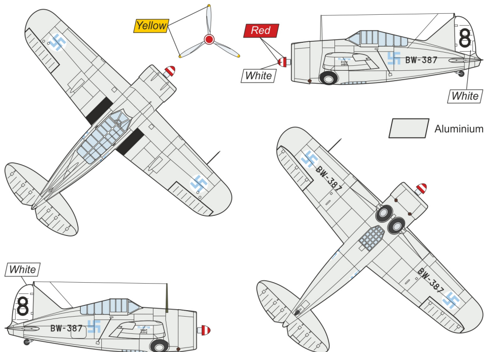
Brewster B-239, Black BW-387/8, LeLv 24, Finnish Air Force, Siikakangas airfield, spring 1941
