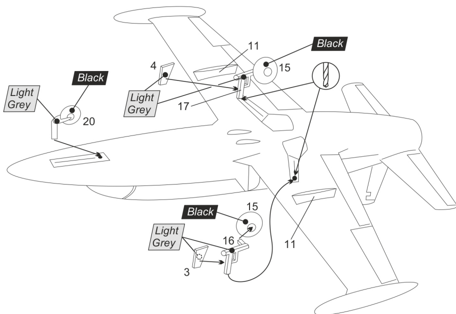
L-39C/ZO underwing pylon location
