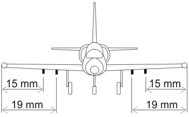
L-39ZO/ZA underwing pylons location
