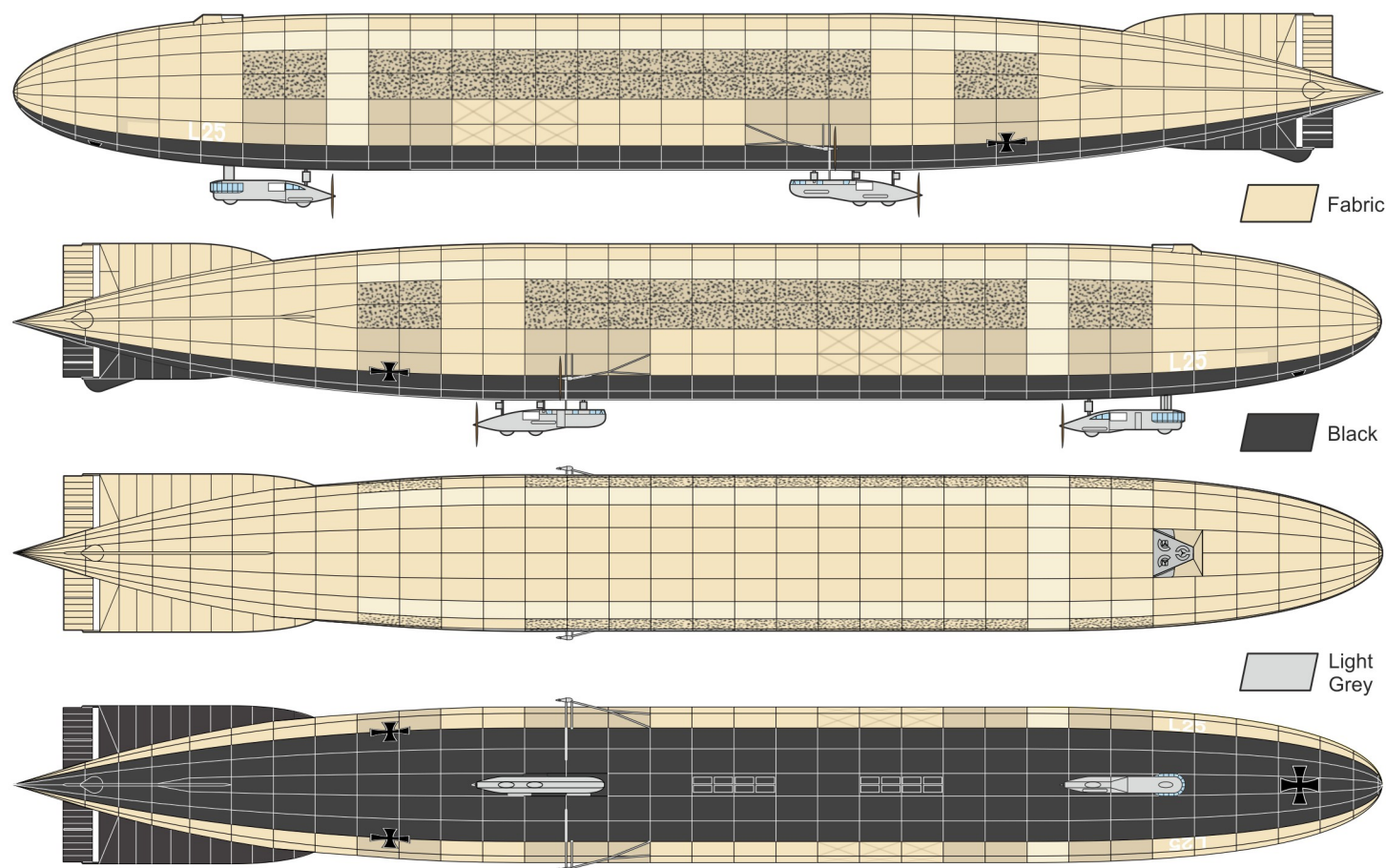
B Zeppelin LZ58 (P-class), LZ58, White L25, Naval Airship Division (Marine-Luftschiff-Abteilung), Imperial German Navy (Kaiserliche Marine), Potsdam Airship Base, Germany, 1917
