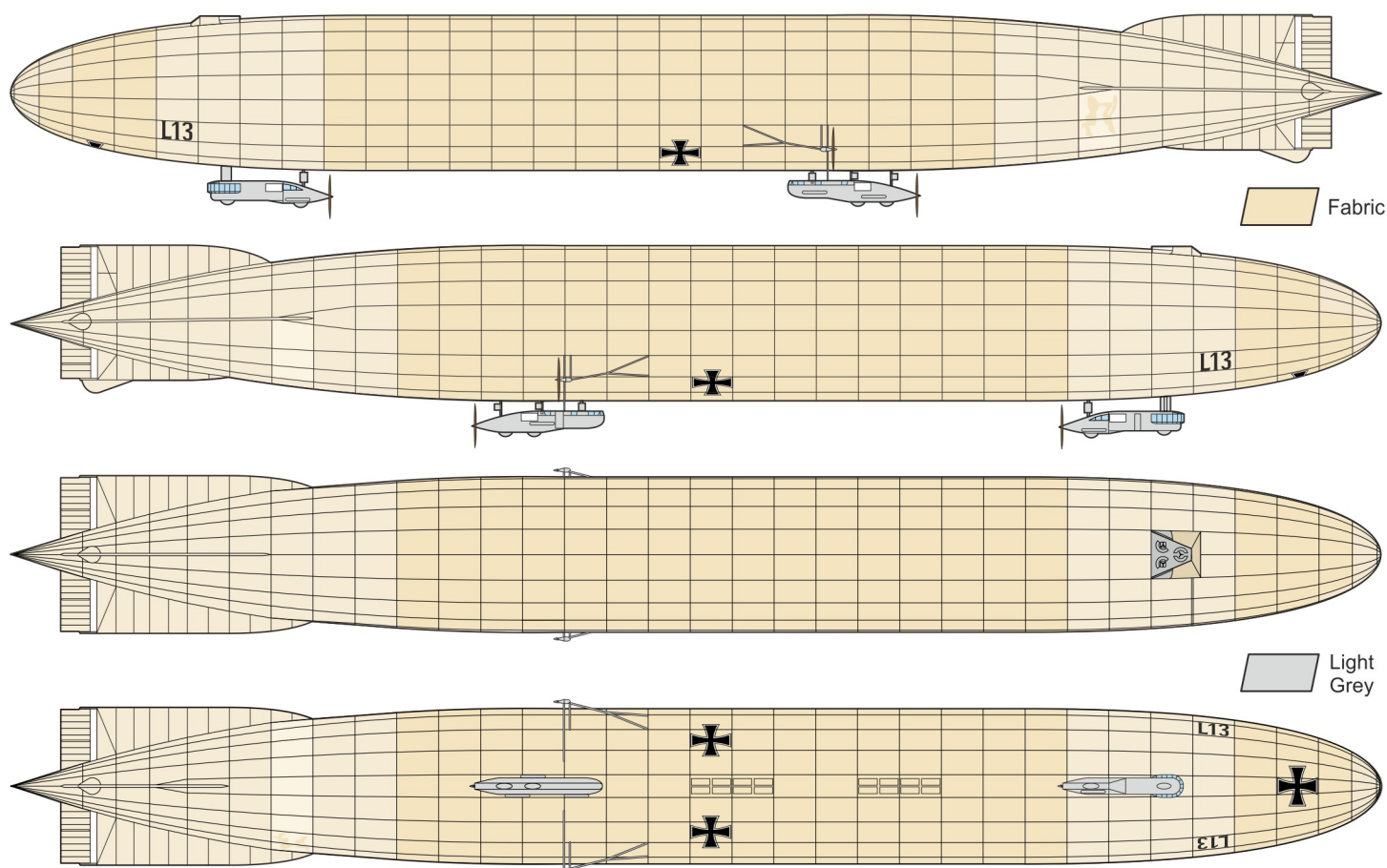
A Zeppelin LZ45 (P-class), L13, Black L13, Naval Airship Division (Marine-Luftschiff-Abteilung), Imperial German Navy (Kaiserliche Marine), Hage Airship Base, Germany, Action of 19 August 1916, summer 1916
